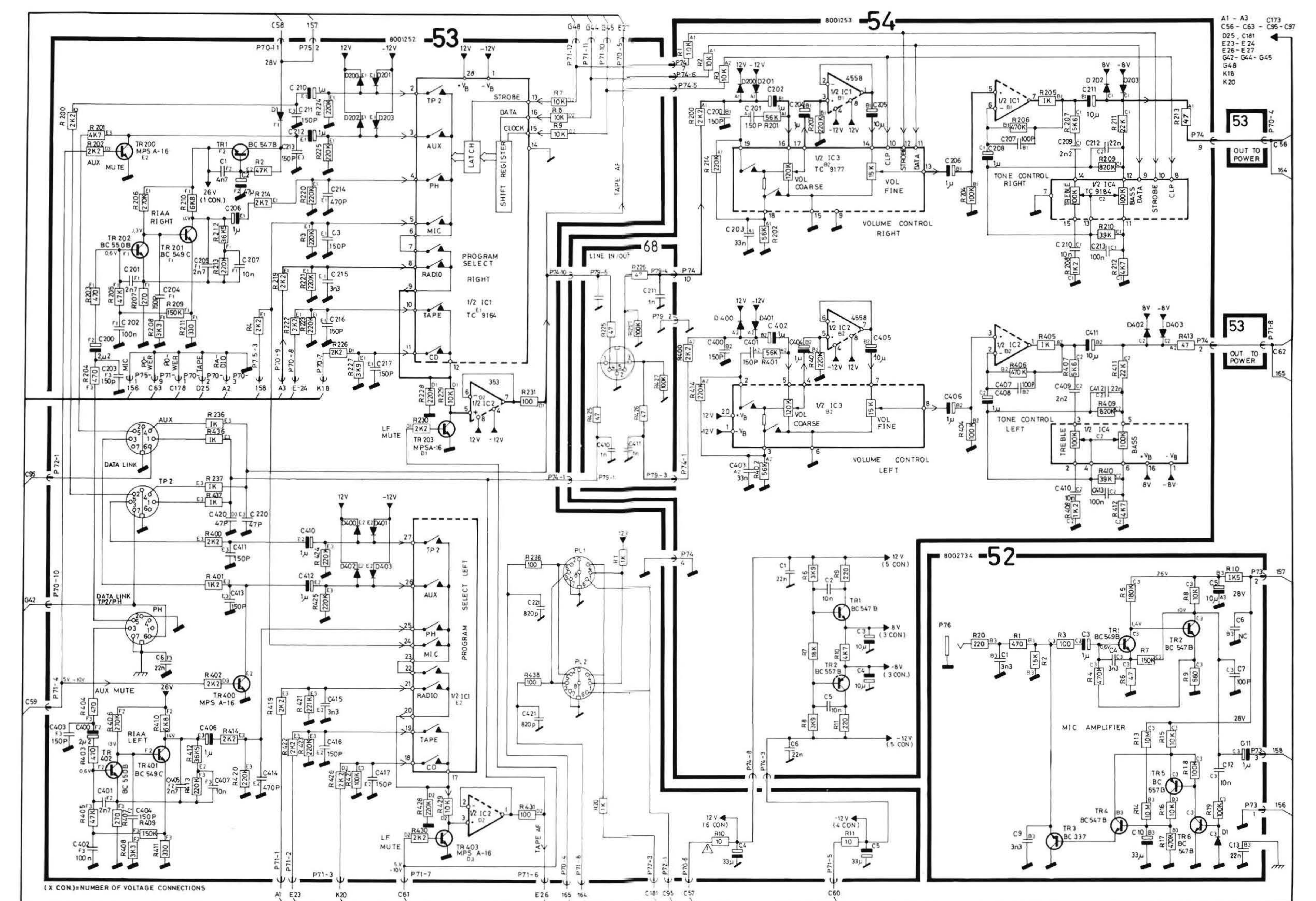
DIAGRAM B (Mic. Ampl., Input Select, Tone and Volume Control)
