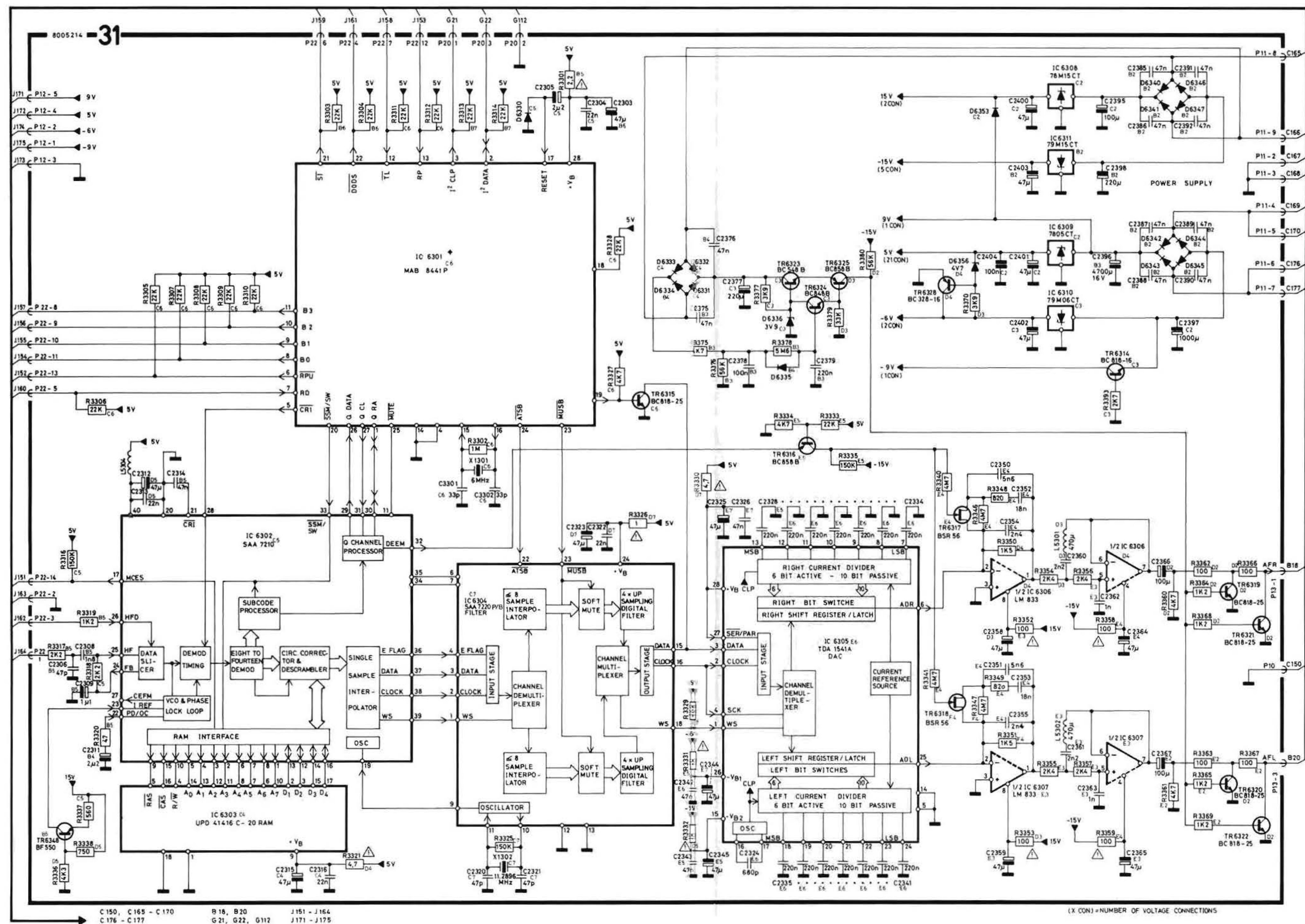
DIAGRAM K (Decoder)
